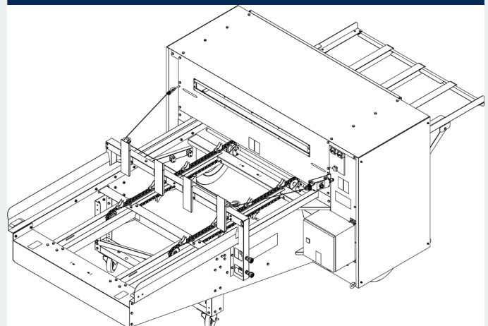
Slat washer for wooden slats
